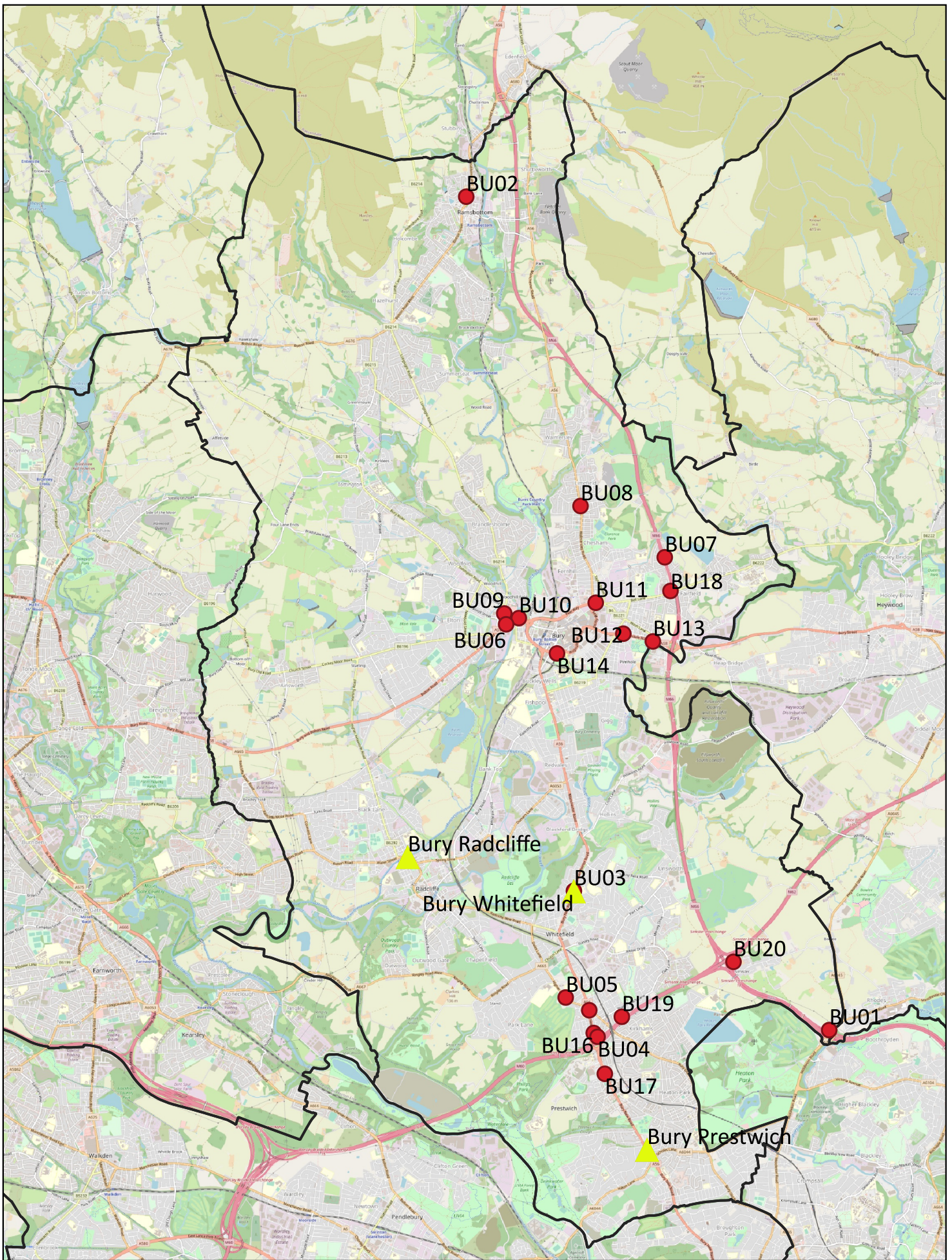
Location of Automatic Monitoring Stations and NOx Tubes 2021 Bury Council Air Quality Monitoring
